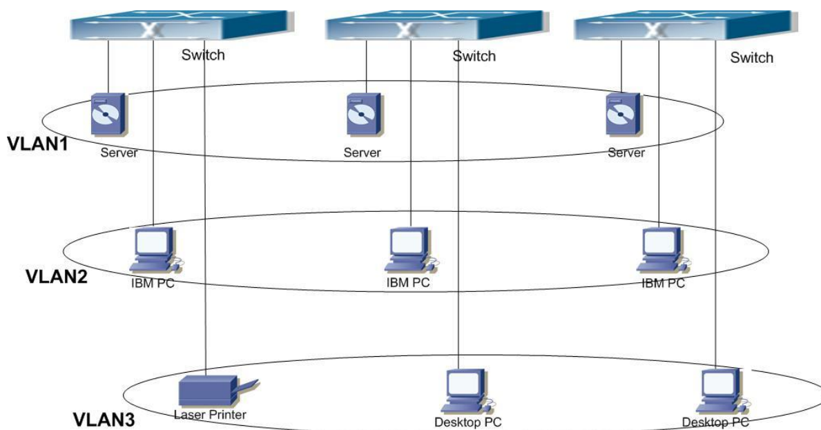
Figure 5-1 Logical definition of the VLAN network
