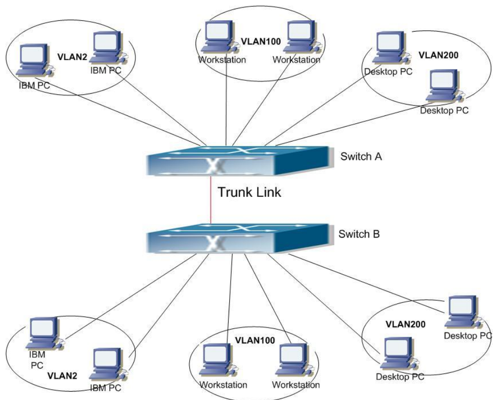
Figure 5-1 VLAN typical application topology
