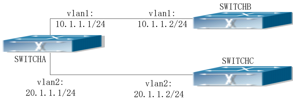
Picture 12-3 OSPF Case
