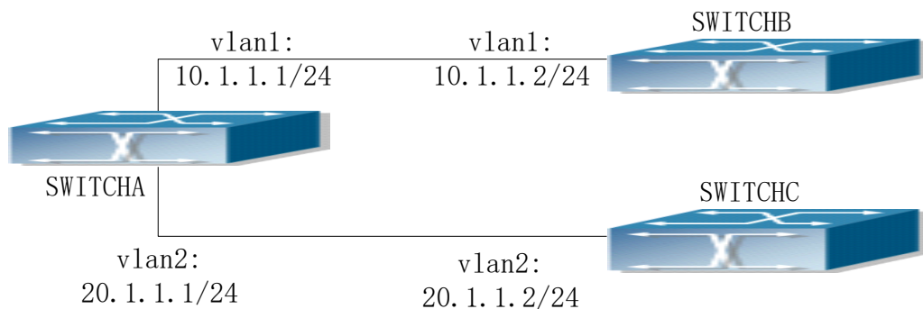
Picture 12-2 RIP Case
