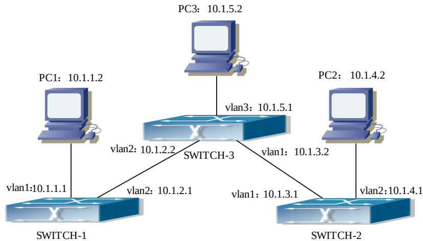
Figure 12-1 Static routing configuration diagram.
