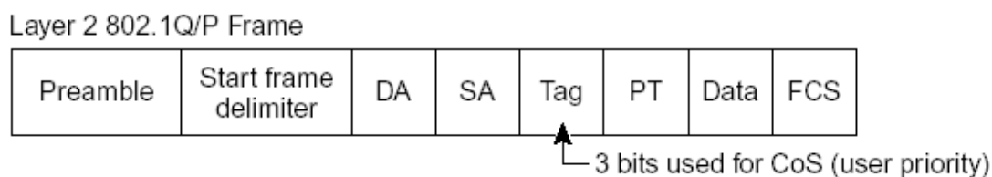
Figure 8-1 CoS Priority
