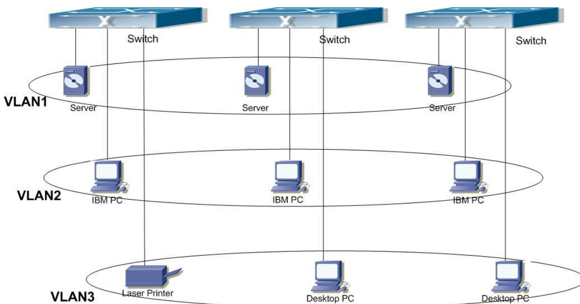
Figure 5-1 Logical definition of the VLAN network
