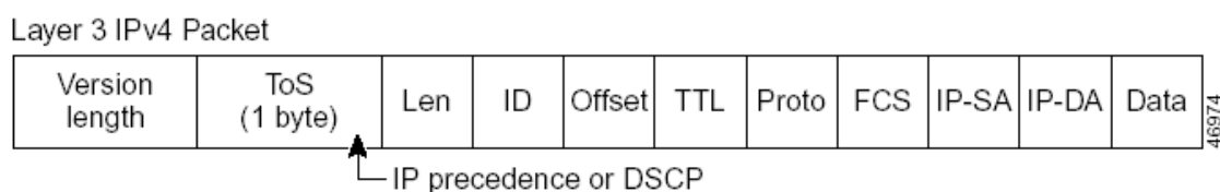
Figure 8-2 ToS Priority
